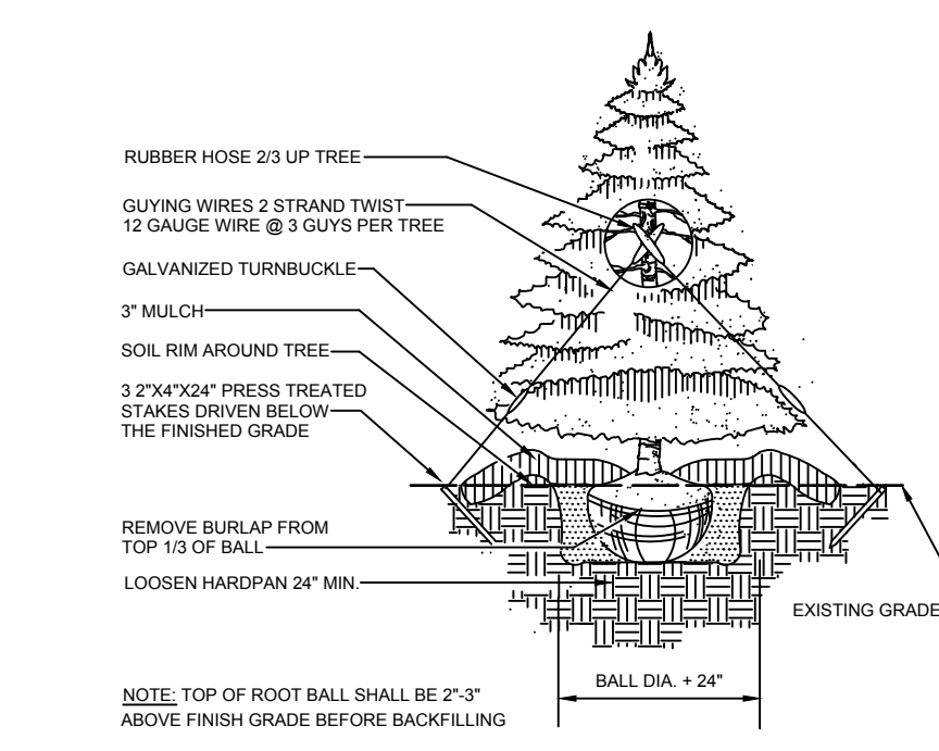
DETAIL: EVERGREEN TREE PLANTING NOT TO SCALE
