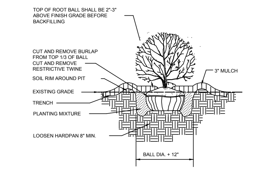
DETAIL: SHRUB PLANTING NOT TO SCALE
