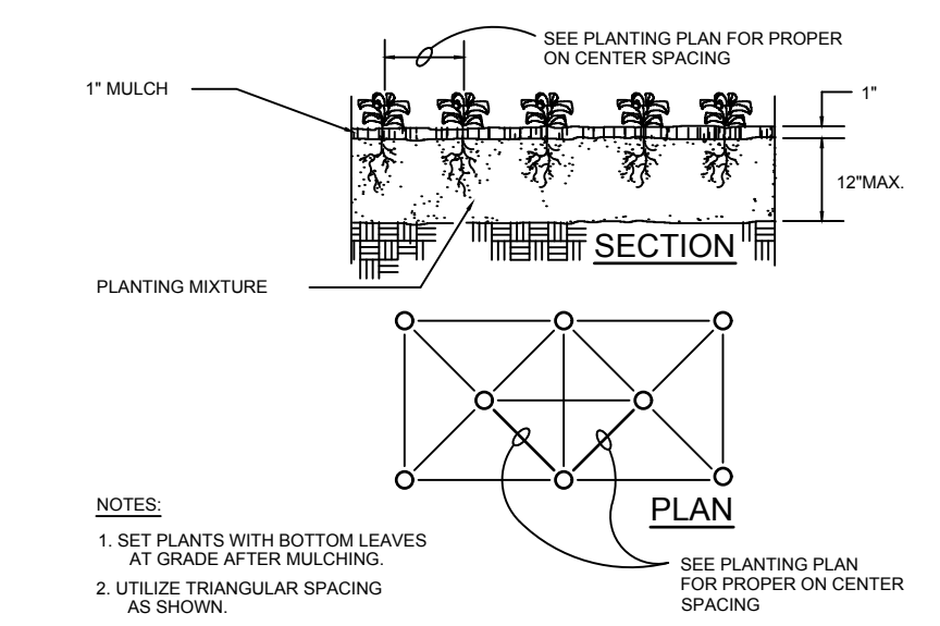
DETAIL: GROUND COVER PLANTING NOT TO SCALE
